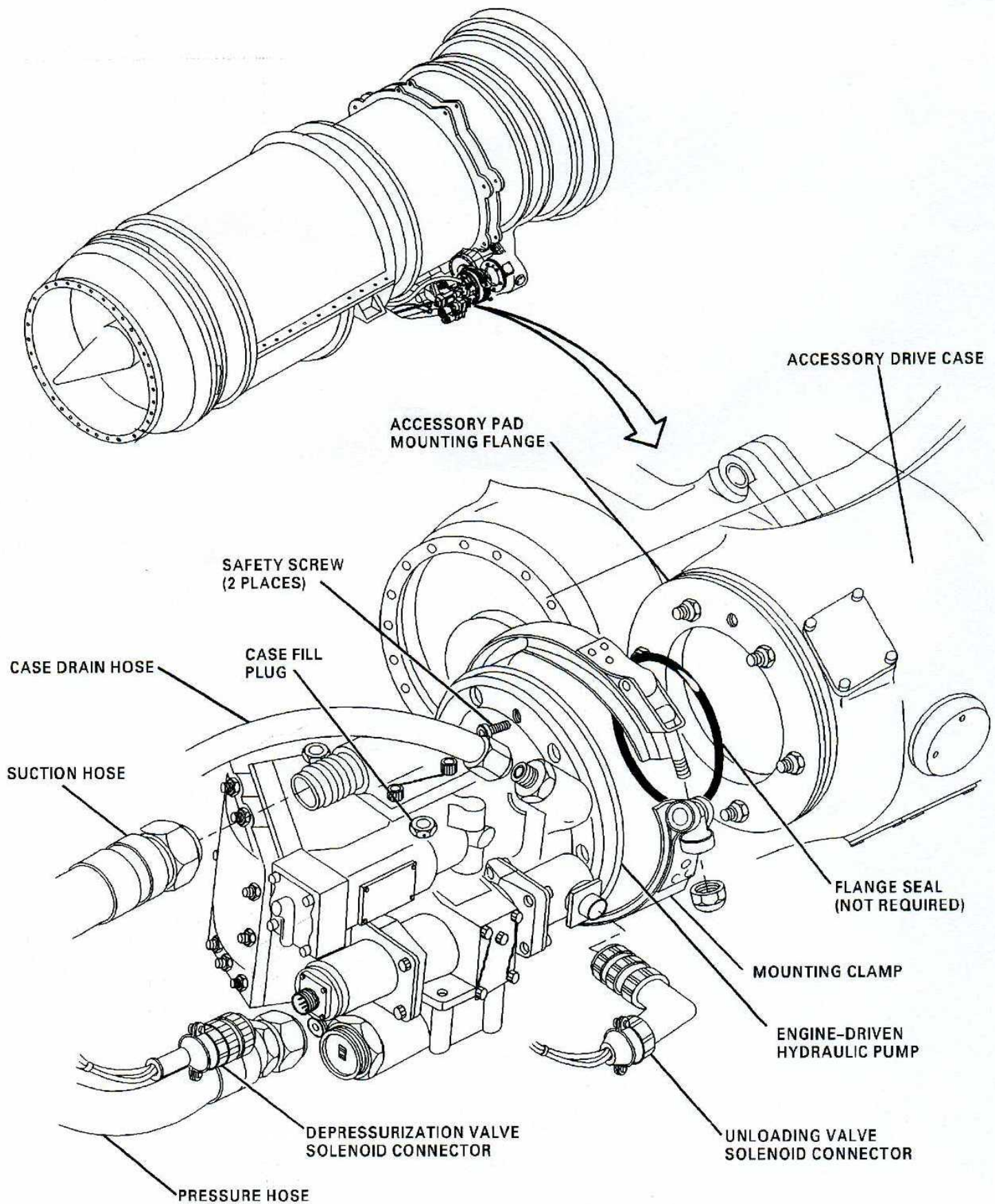
Engine-Driven Hydraulic Pump -- Removal/Installation Figure 201 (sheet 1)
